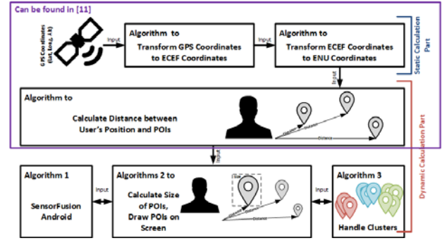
Fig. 3. Algorithm Dependencies
