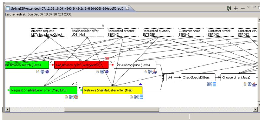
Abb. 11 Process Monitor: Monitoring Perspective
