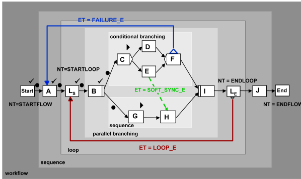
Abb. 4 ADEPT Process Meta Model
