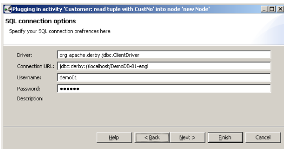
Abb. 9 Setting connection details in a DB activity template
