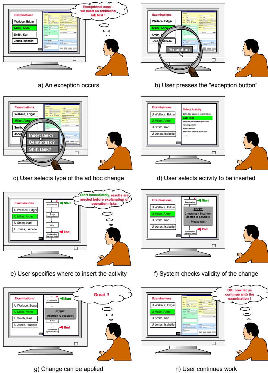
Abb. 3 Executing an ad hoc modification from the end-user's point of view
