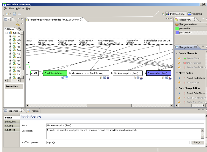
Abb. 12 Process Monitor: Instance Change Perspective
