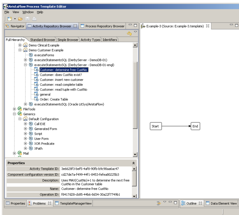
Abb. 8 Activity Repository Browser window in the Process Template Editor
