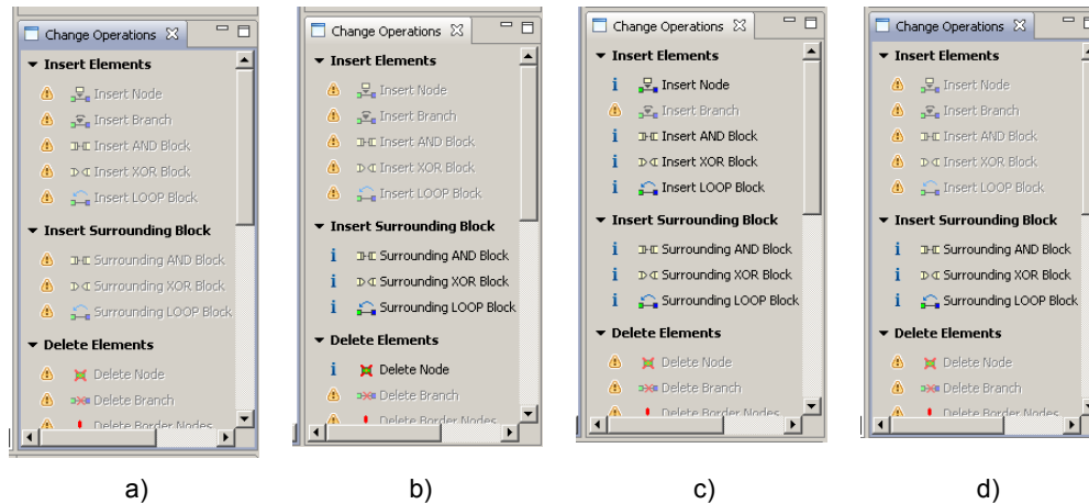
Abb. 6 Enabled change operations
