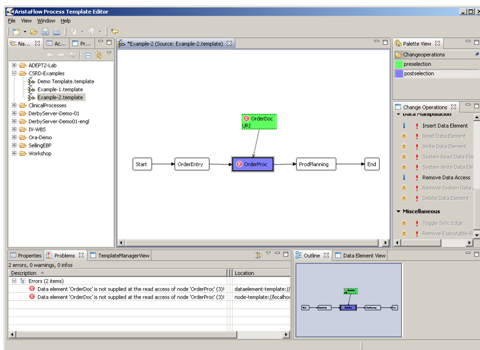
Abb. 7 Reporting of detected deficiencies (problem window on the left at the bottom)
