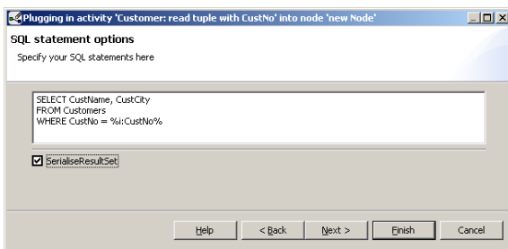
Abb. 10 DB activity template with defined SQL statement
