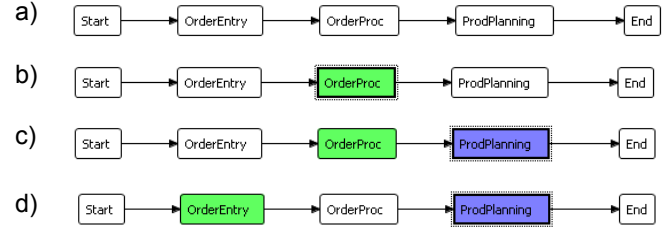
Abb. 5 Markings in the process graph
