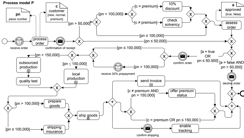
Fig. 1. An order-to-delivery process (modeled with BPMN)
