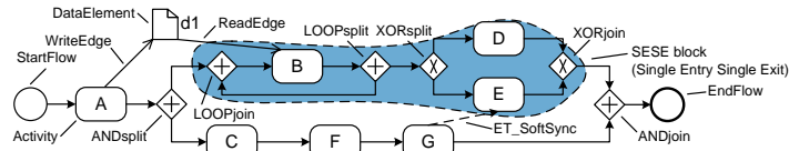
Fig. 2: Example of a Process Model
