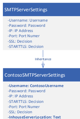
Figure 3.2.: Inheritance Example
