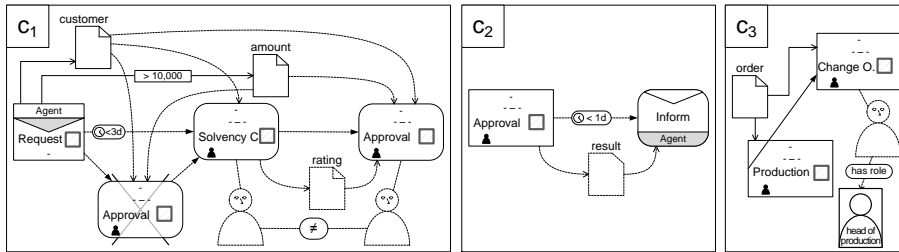
Fig. 4: Modeling compliance rules c_1 - c_3 with the eCRG language
