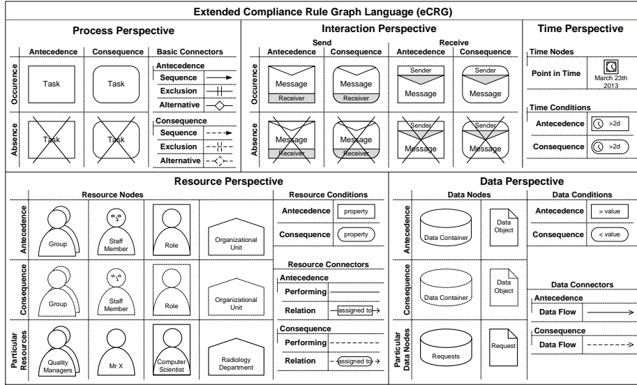
Fig. 3: Elements of the eCRG language
