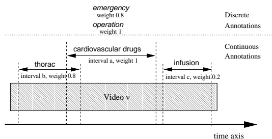
Figure 2: Video v with discrete and continuous annotations
