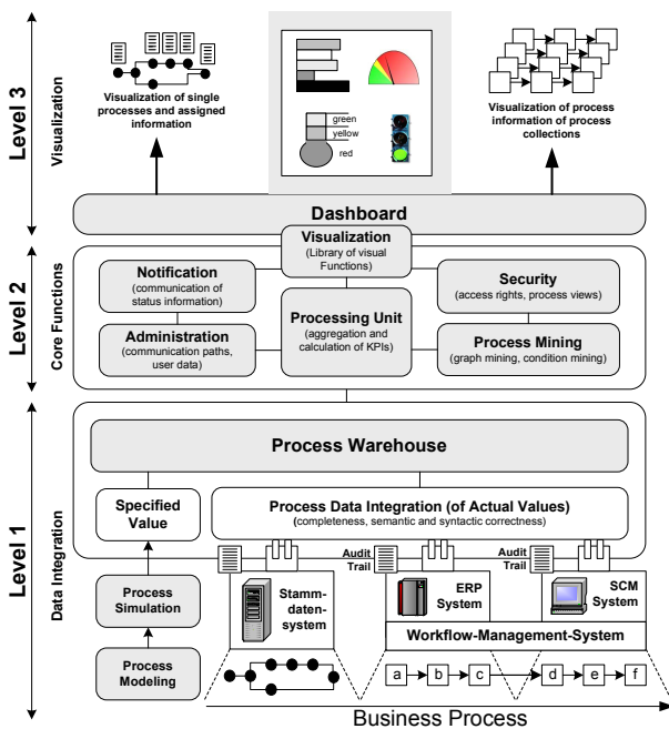
Figure 14. Reference Architecture.
