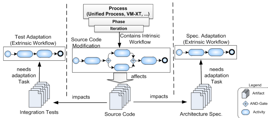
Fig. 1. Intrinsic and Extrinsic Workflows.
